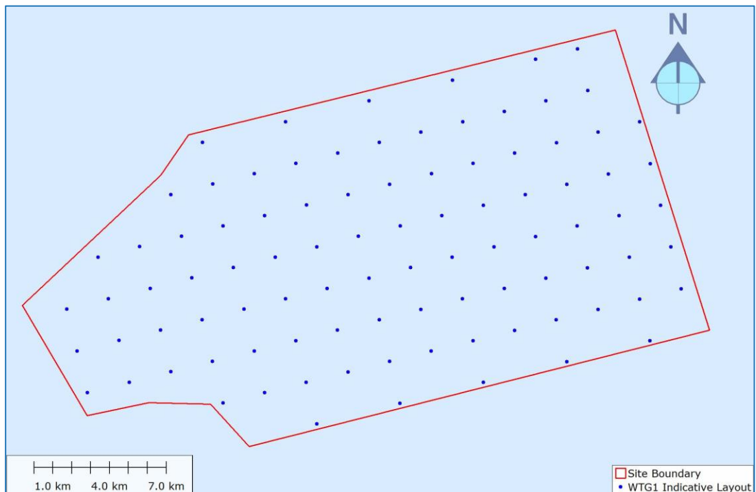
Figure 1: WTG1 indicative layout – 93 WTGs
