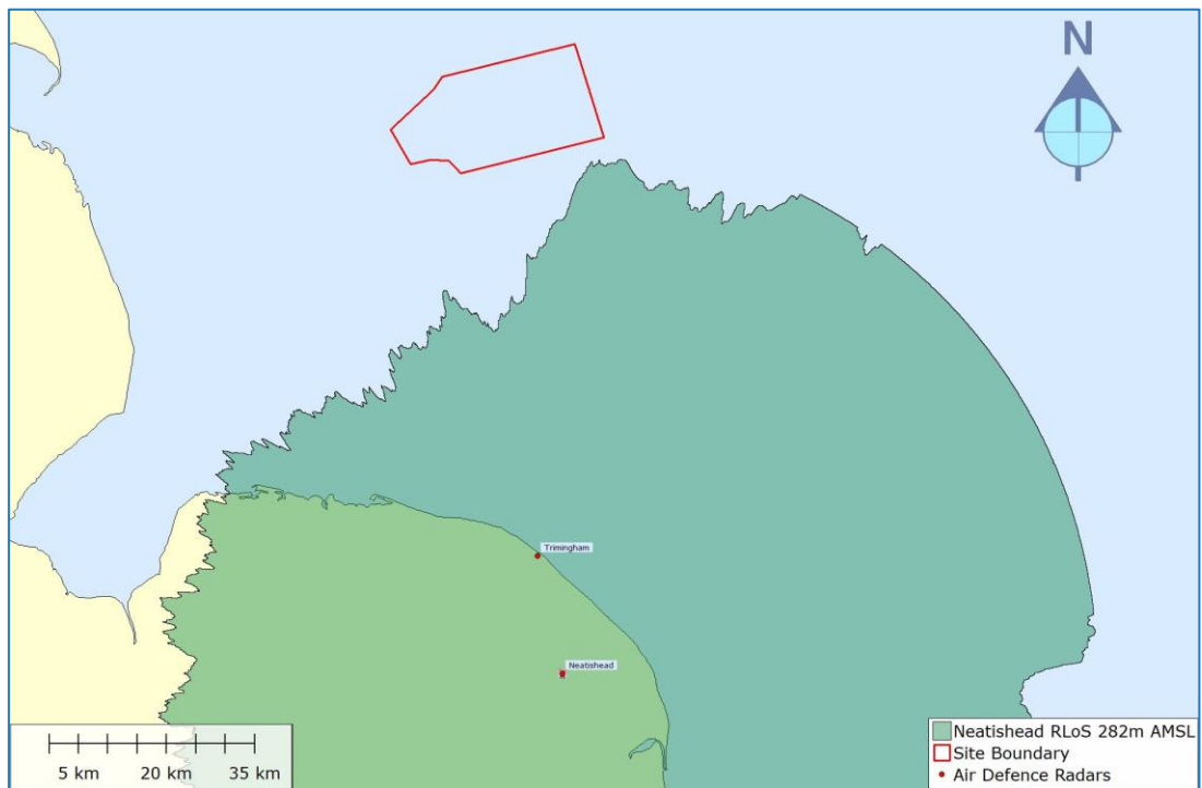
Figure 27: Neatishead RLoS 282m AMSL
