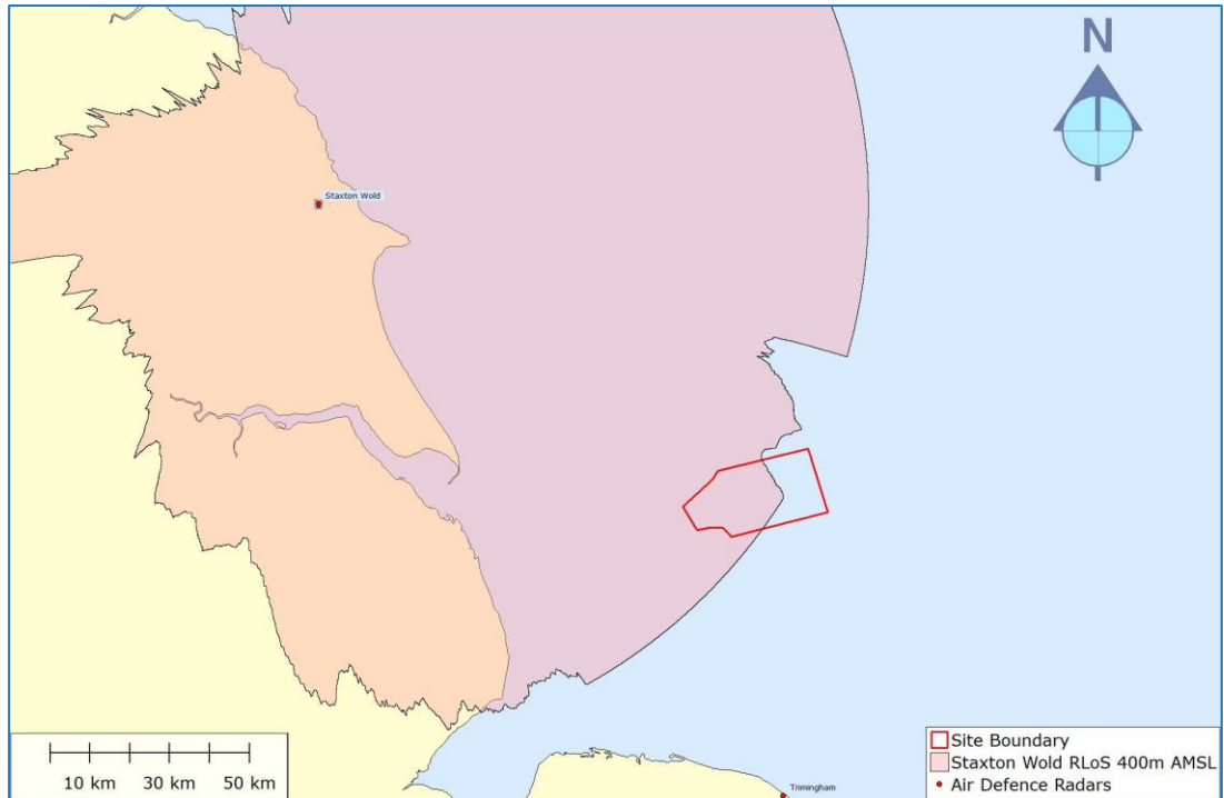
Figure 22: Staxton Wold RLoS 400m AMSL
