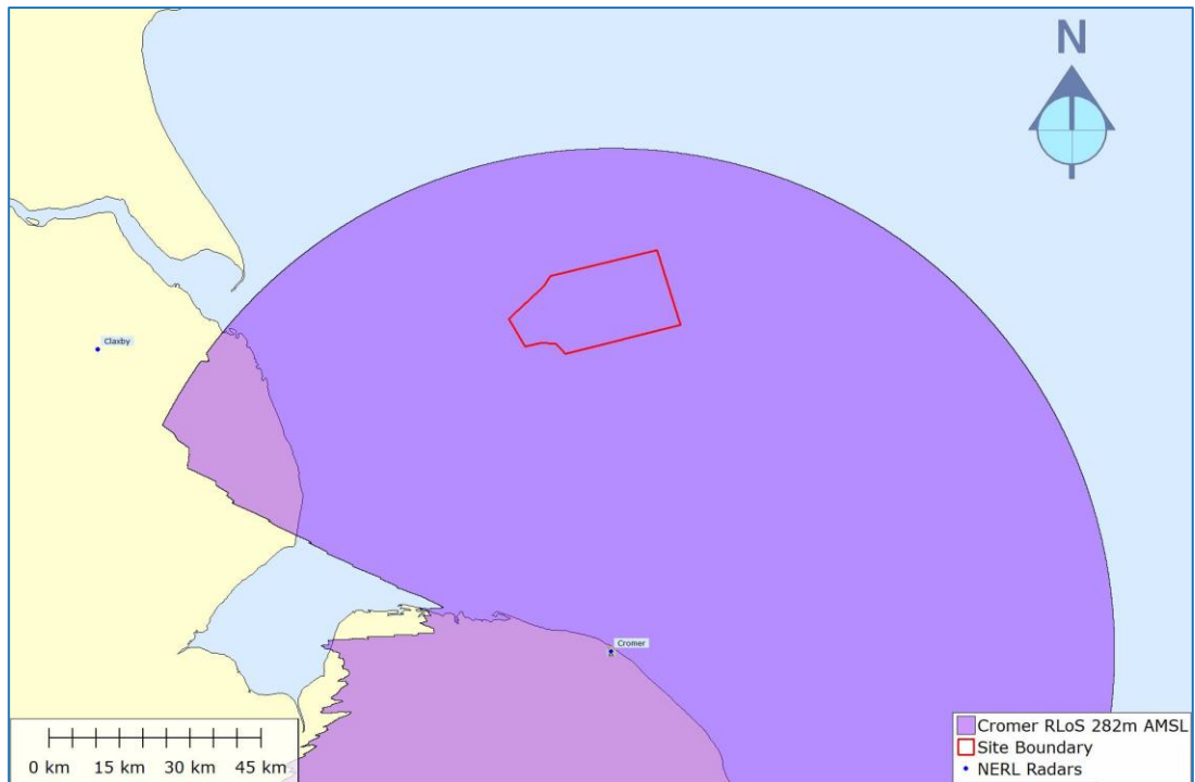
Figure 21: Cromer RLoS 282m AMSL
