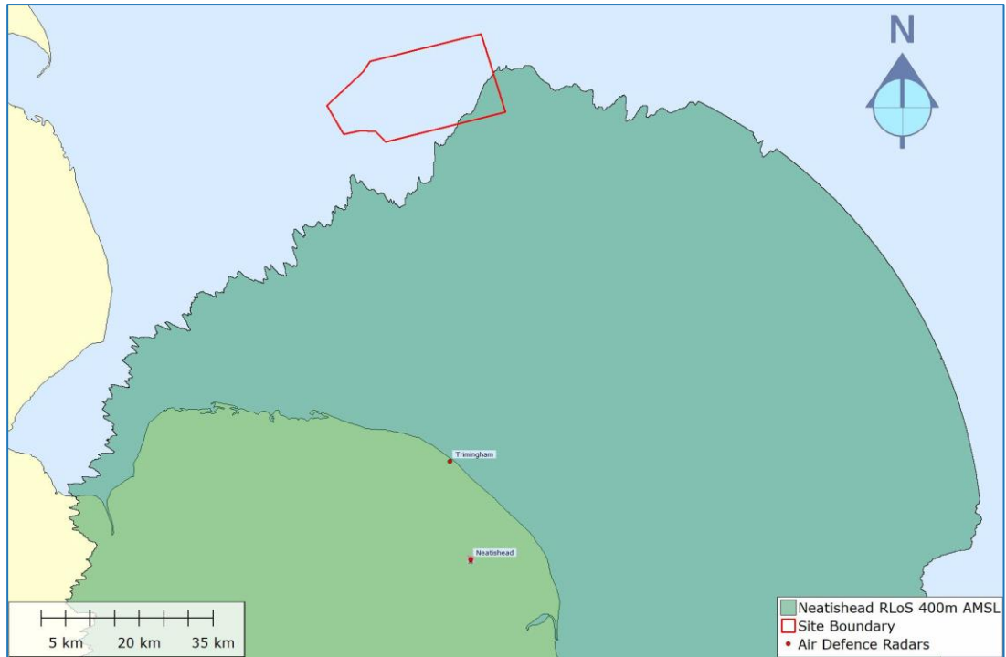
Figure 26: Neatishead RLoS 400m AMSL
