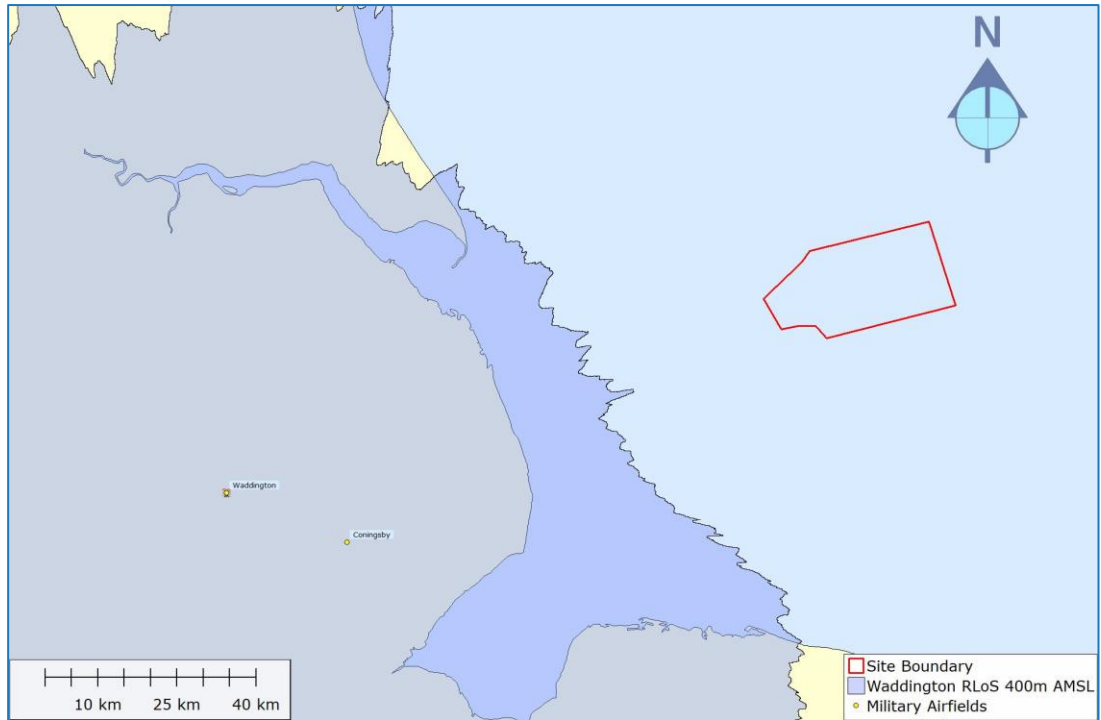
Figure 17: Waddington RLoS 400m AMSL
