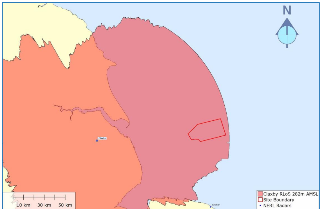
Figure 19: Claxby RLoS 282m AMSL
