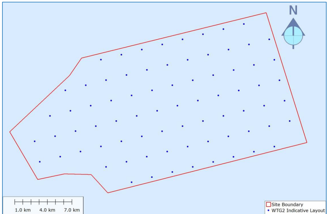
Figure 2: WTG2 indicative layout – 75 WTGs
