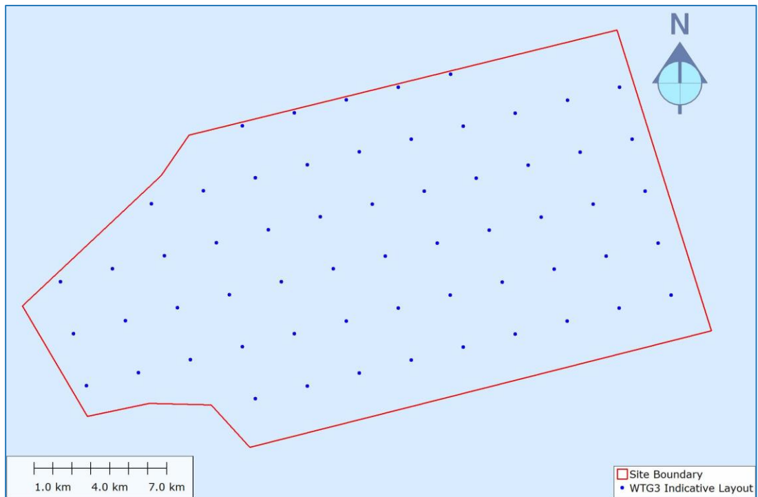
Figure 3: WTG3 indicative layout – 60 WTGs
