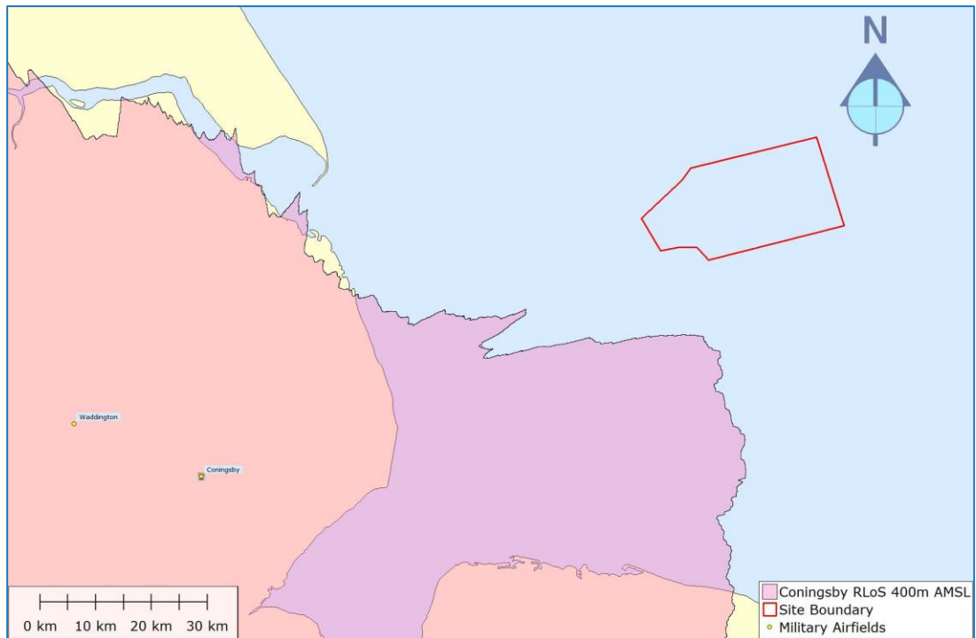
Figure 15: Coningsby RLoS 400m AMSL
