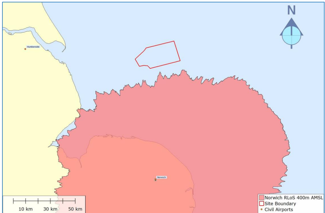
Figure 14: Norwich RLoS 400m AMSL
