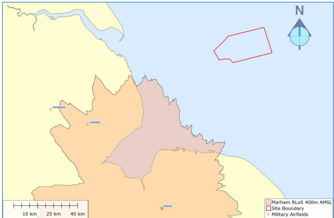
Figure 16: Marham RLoS 400m AMSL
