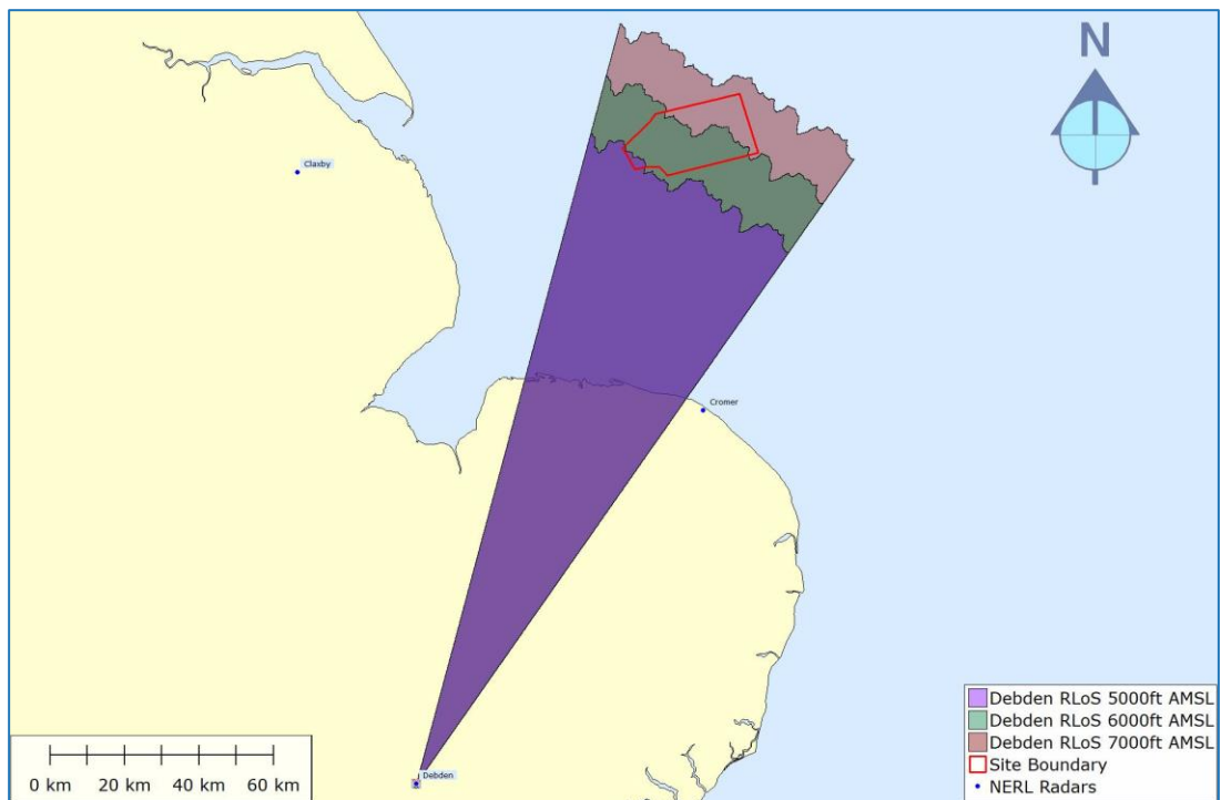
Figure 28: Debden RLoS coverage at 5,000ft, 6,000ft and 7,000ft AMSL
