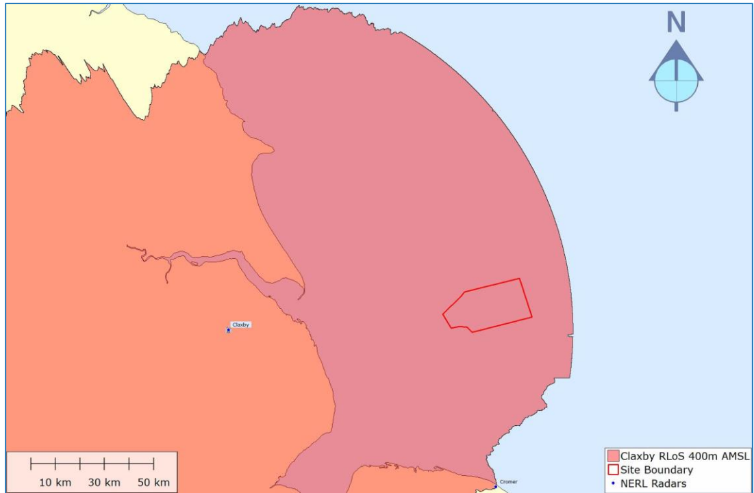
Figure 18: Claxby RLoS 400m AMSL
