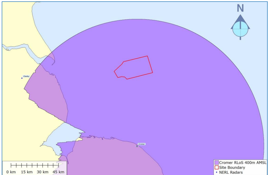
Figure 20: Cromer RLoS 400m AMSL
